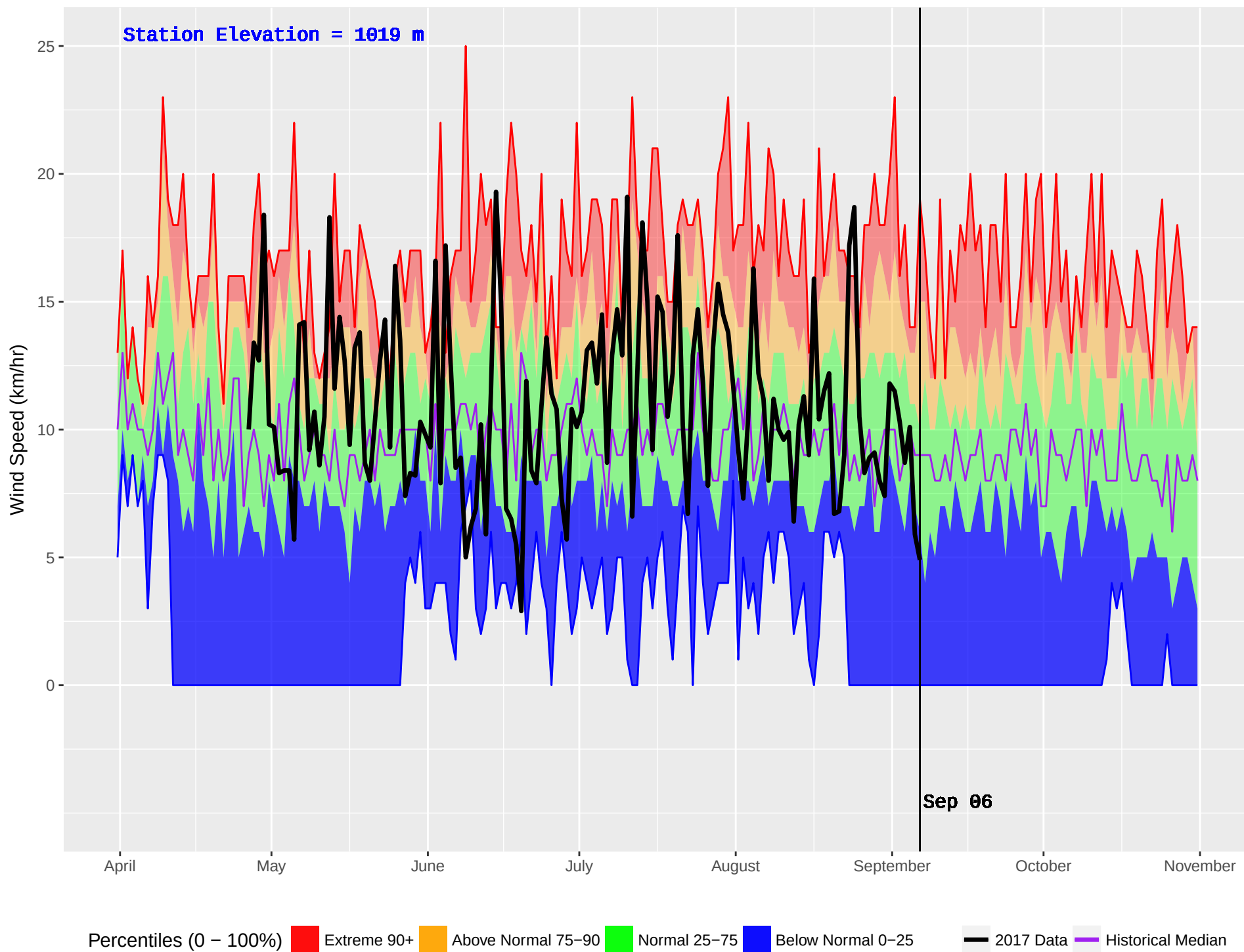
POWDER CREEK (380) : Historical (2001–2016) and Current (2017) Noon Wind Speed
